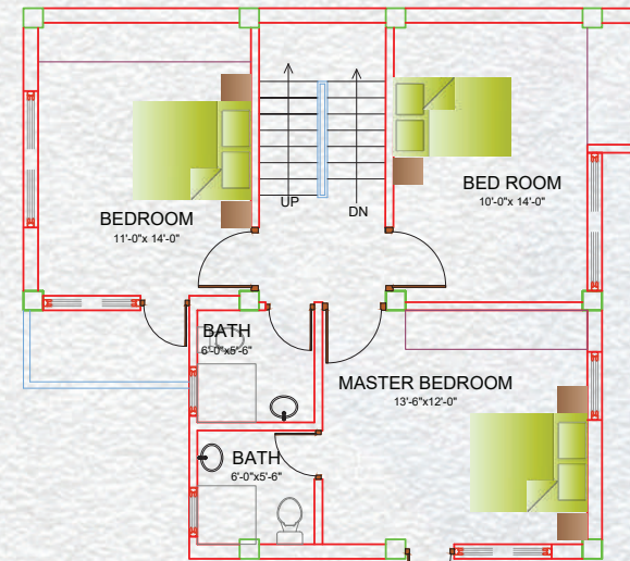
FIRST FLOOR PLAN Area: 782 sq.ft
