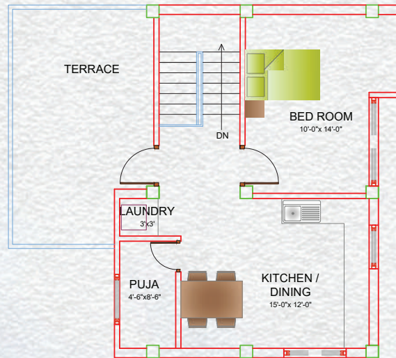
SECOND FLOOR PLAN Area: 576 sq.ft
